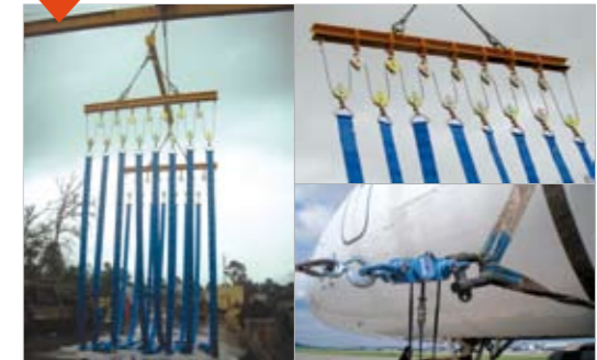
Spreader Bar Tethering -Towing
